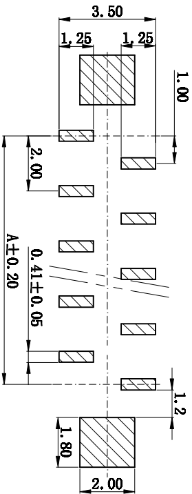
PCB layout
